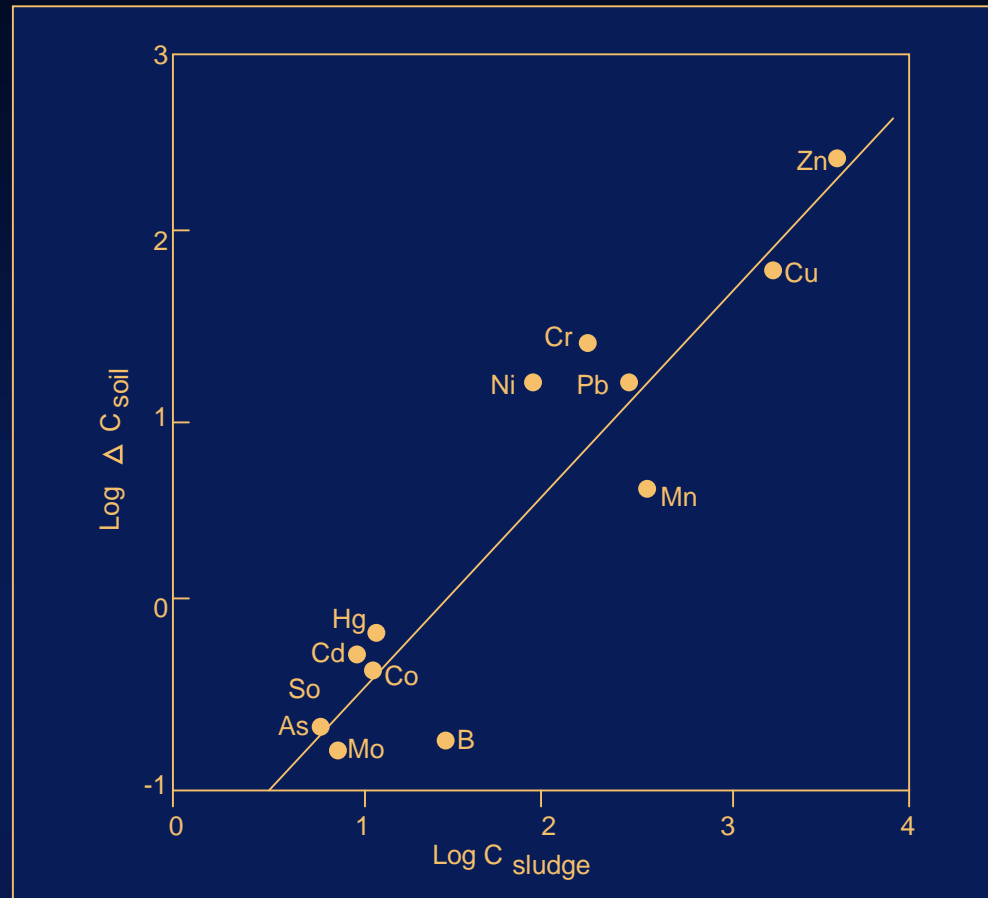
Relationship between concentration of trace elements in sewage sludge ( C_{\text{sludge}} ) and the increase of trace elements in the soil ( C_{\text{soil}} ) from using sewage Sludge. Source: Andersson and Nilsson, 1972.
