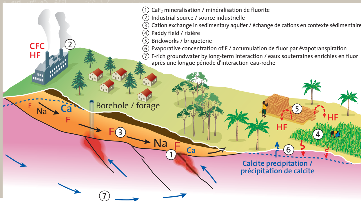
◀ Fig. 2: Schematic diagram showing fluoride-concentrating factors in sedimentary and granite contexts..
