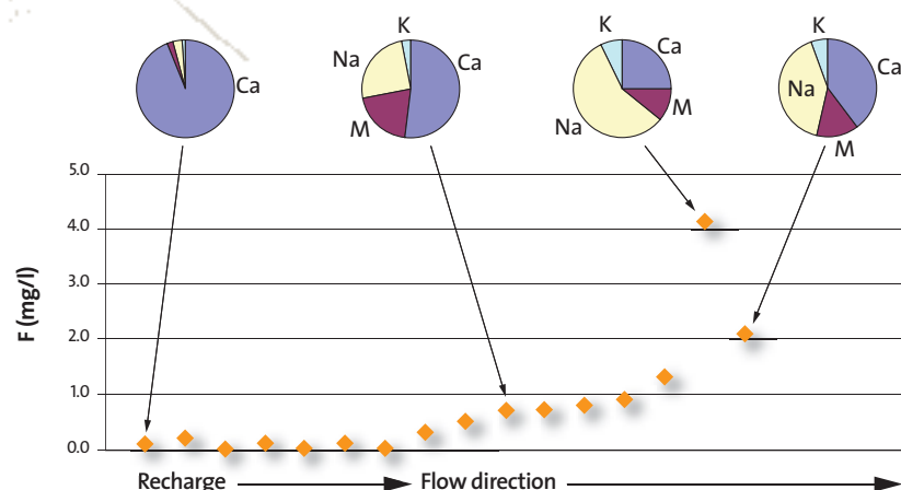
Fig. 3: Evolution of fluoride concentrations in groundwater from a Jurassic limestone aquifer (southwestern France) according to the covered distance. Pie charts illustrate the increase of sodium (Na) and decrease of calcium (Ca) concentrations with fluoride increase.
