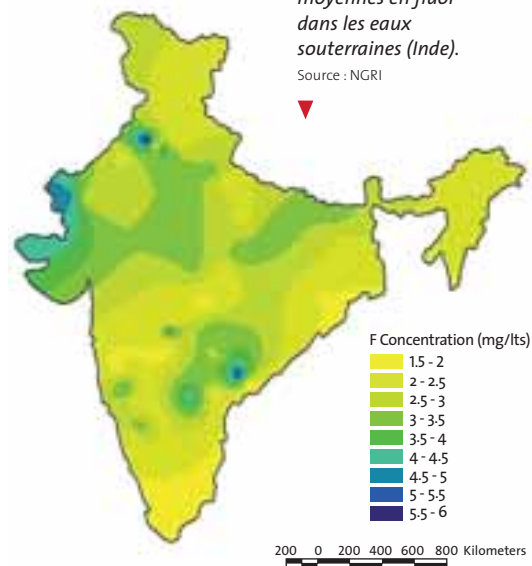
Fig. 1: Map of mean fluoride concentrations in Indian groundwater.
