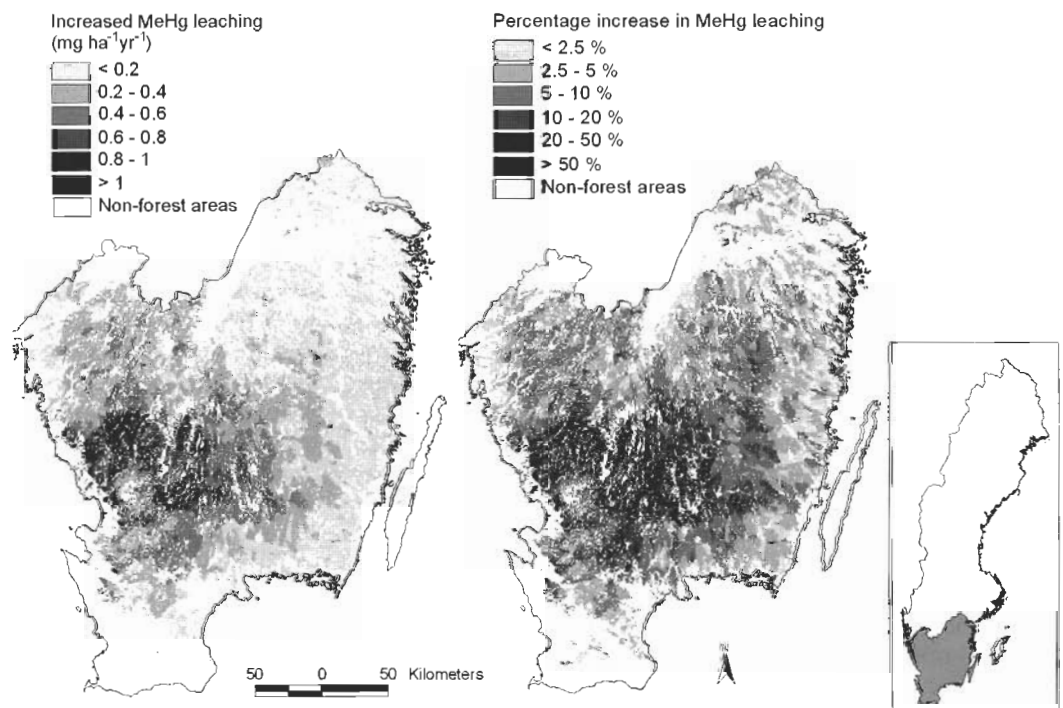
Figure 1. Modeled increased levels of MeHg following the 2005 storm event in SW Sweden (average values during a period of about 5 years).
