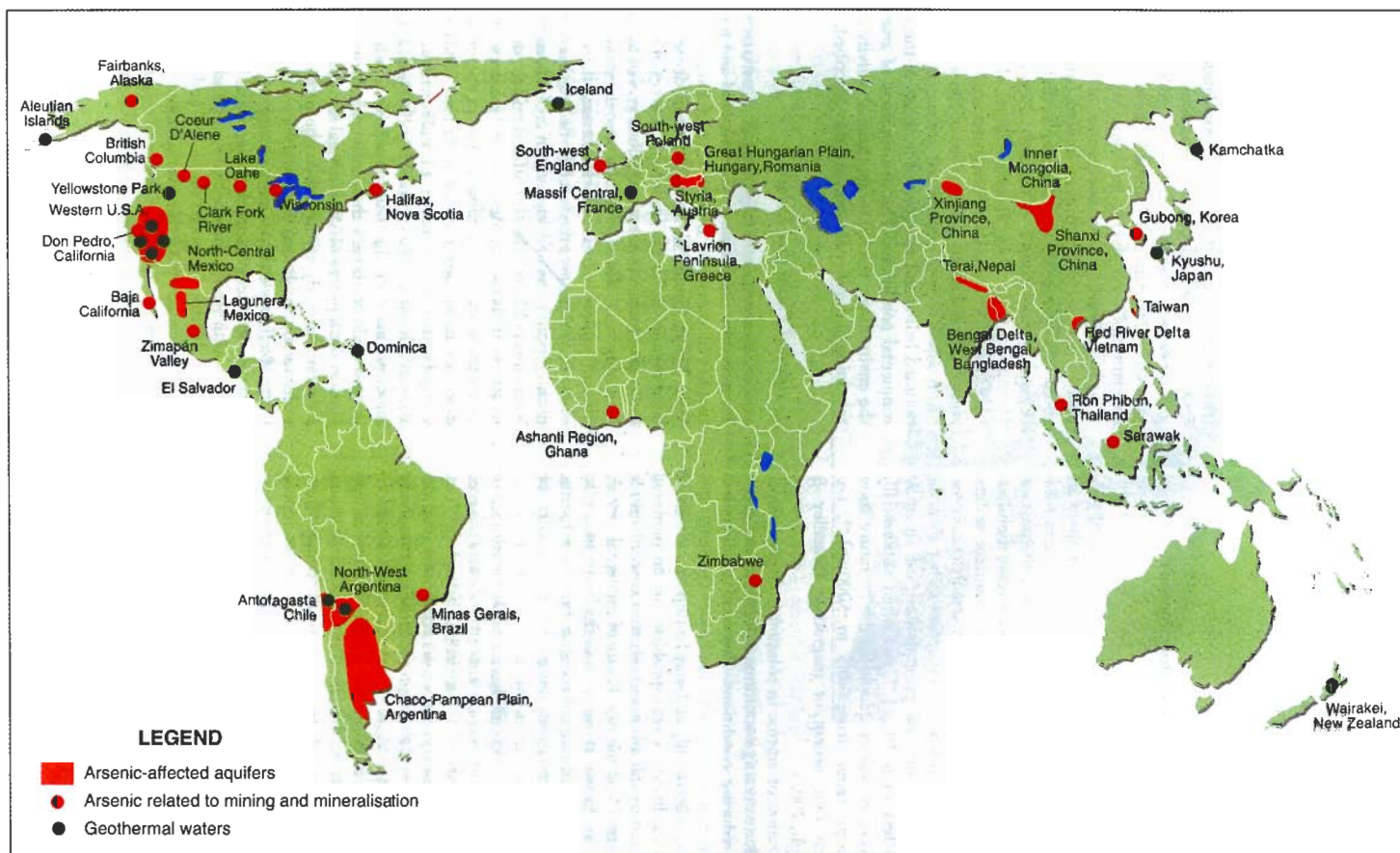
Figure 1. World map illustrating regions with documented arsenic problems in groundwater ( As > 50 \mu g L^{-1} ). Adapted from Ref. 22.
